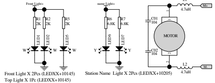
Front Light X 2Pcs (LEDXX+10145) Top Light X 1Pc (LEDXX+10145) Station Name Light X 2Pcs (LEDXX+10205) Interior Light x 8Pcs Rear Light X 2Pcs (LEDXX+10175) Interior Light X 6Pcs (LEDXX+10205)
