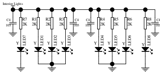
Interior Light x 8Pcs
